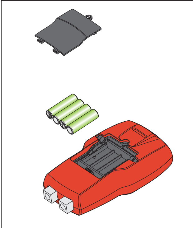
Figure 8. Battery Replacement
