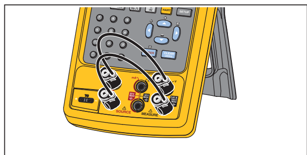
Figure 2. Jumper Connections
