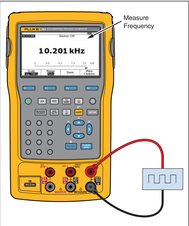
Figure 51. Tachometer Examination
