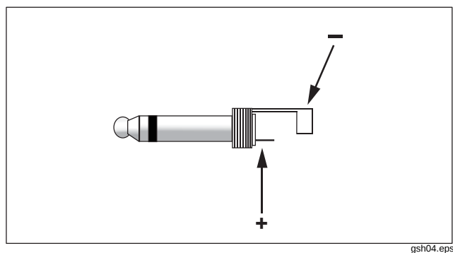
Figure 2. External Trigger Connector Polarity
