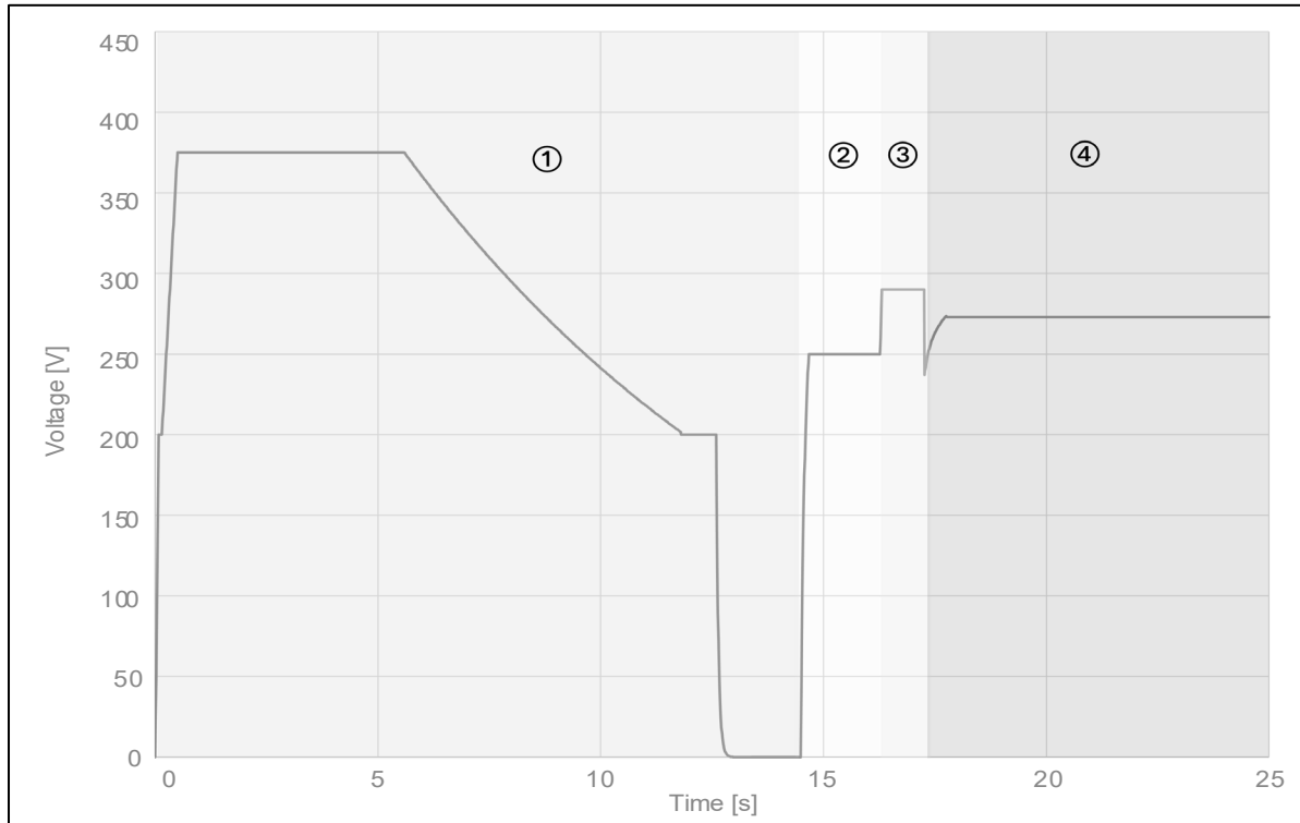
Figure 1. Performing Load Test
