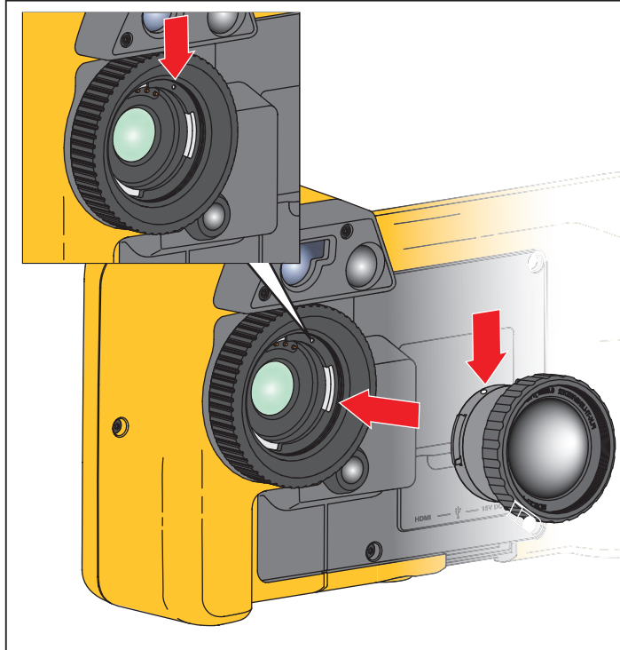
Figure 2. Optional Lens Installation
