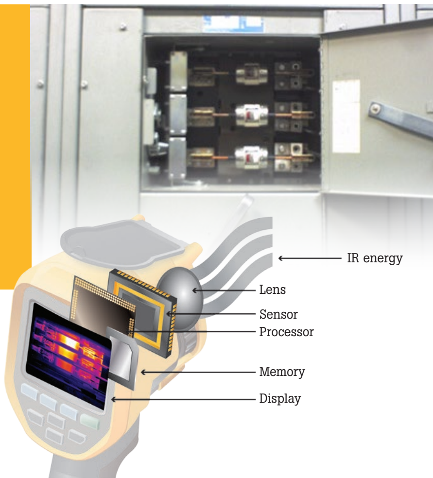
Figure 1. Anatomy of an infrared camera
